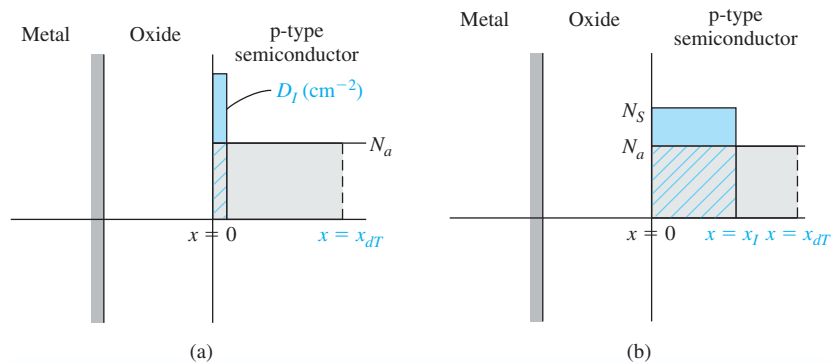
Figure 11.29 | (a) Ion-implanted profile approximated by a delta function. (b) Ion-implanted profile approximated by a step function in which the depth x_I is less than the space charge width x_{dr} .
