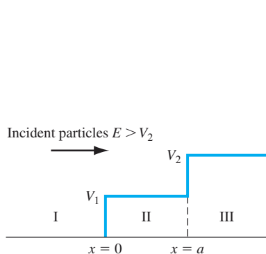
Figure P2.39 | Potential function for Problem 2.39.
