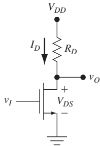
Figure 15.26 | A MOSFET inverter circuit.
