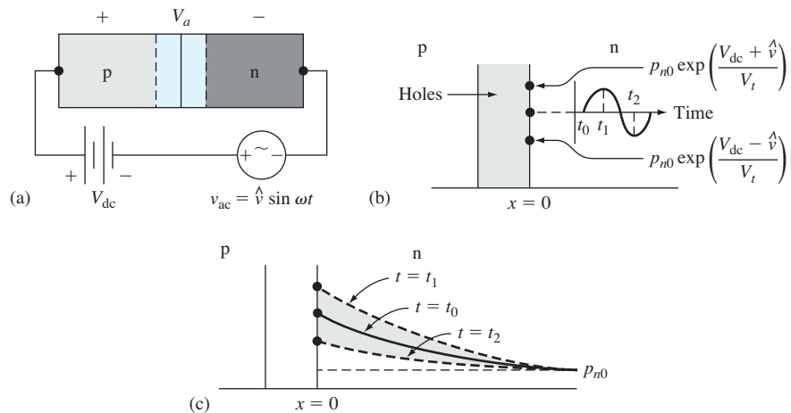
Figure 8.19 (a) A pn junction with an ac voltage superimposed on a forward-biased dc value; (b) the hole concentration versus time at the space charge edge; (c) the hole concentration versus distance in the n region at three different times.
