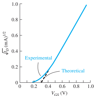
Figure 13.14 | Experimental and theoretical \sqrt{I_D} versus V_{GS} characteristics of an enhancement mode JFET.
