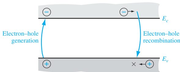
Figure 6.1 | Electron-hole generation and recombination.
