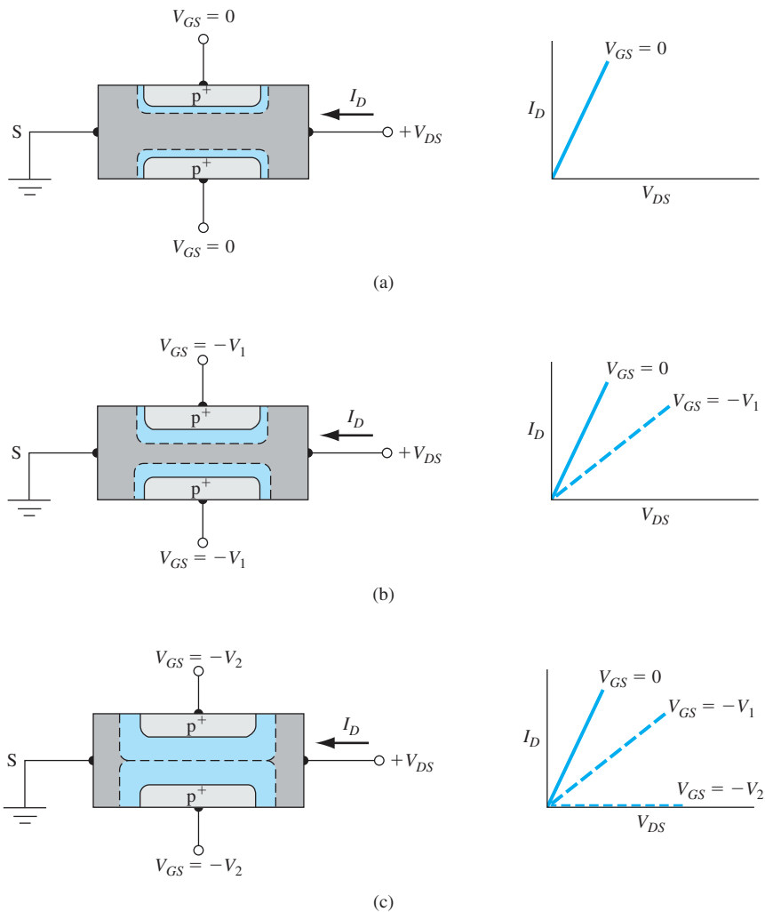
Figure 13.3 | Gate-to-channel space charge regions and I - V characteristics for small V_{DS} values and for (a) zero gate voltage, (b) small reverse-biased gate voltage, and (c) a gate voltage to achieve pinchoff.
