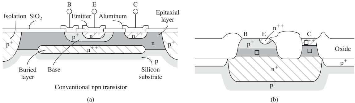
Figure 12.2 | Cross section of (a) a conventional integrated circuit npn bipolar transistor and (b) an oxide-isolated npn bipolar transistor.
