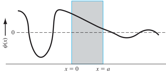
Figure 2.10 | The wave functions through the potential barrier.
