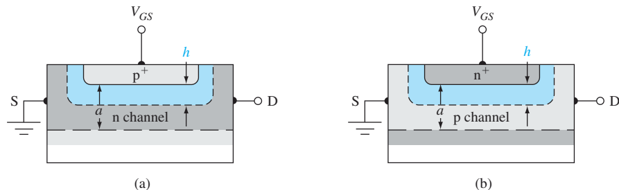
Figure 13.10 | Geometries of simplified (a) n-channel and (b) p-channel pn JFETs.
