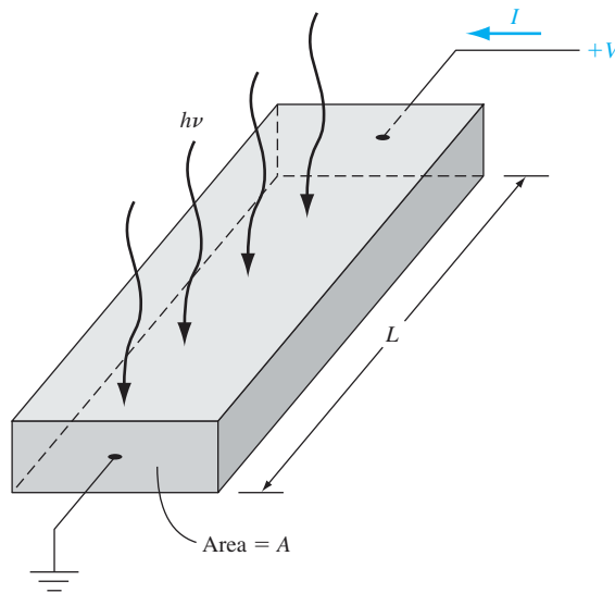
Figure 14.16 | A photoconductor.
