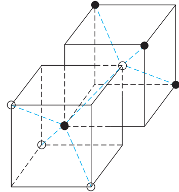
Figure 1.15 | The tetrahedral structure of closest neighbors in the zincblende lattice.
