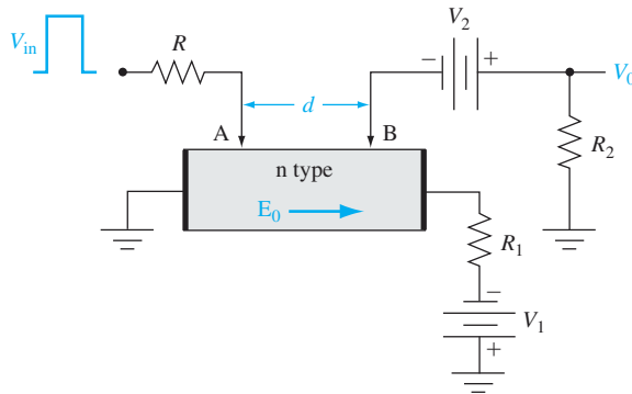
Figure 6.11 | The basic Haynes–Shockley experimental arrangement.
