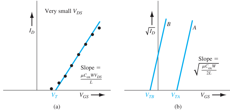
Figure 10.48 | (a) I_D versus V_{GS} (for small V_{DS} ) for enhancement mode MOSFET. (b) Ideal \sqrt{I_D} versus V_{GS} in saturation region for enhancement mode (curve A) and depletion mode (curve B) n-channel MOSFETs.
